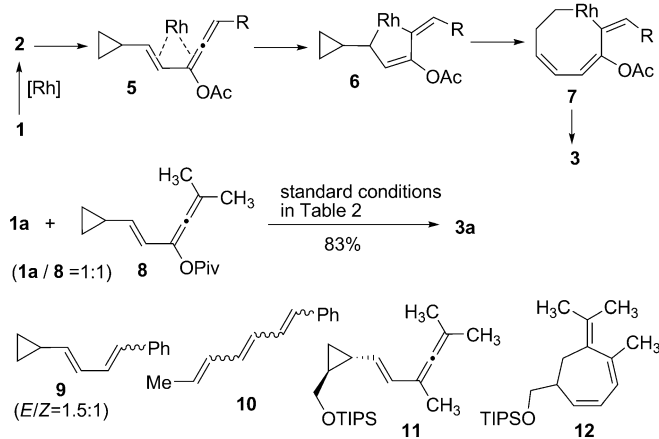
Scheme 1. Proposed mechanism and related evidence.
